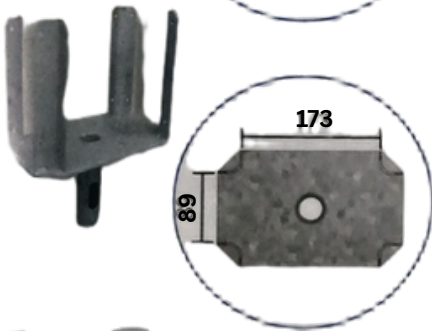
HEAD FOR FORMWORK PROP, HEAVY
